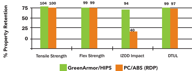
Figure 1 - Multi-Pass Recycle Evaluation From 1st to 5th Injection Molding of HIPS Containing Earthwise GreenArmor and Commercial PC/ABS Formulations
