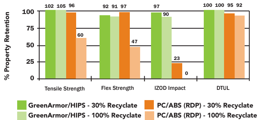
Figure 3 - Extended Heat & Humidity Recycle (30% & 100% Humid Aged Recyclate) of HIPS Containing GreenArmor and Commercial PC/ABS (RDP) - % Property Retention
