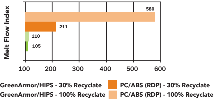
Figure 4 - Extended Heat & Humidity Recycle (30% & 100% Humid Aged Recyclate) HIPS Containing GreenArmor and Commercial PC/ABS Formulations - % Property Retention
