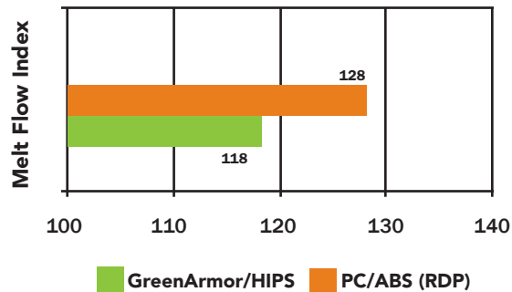
Figure 2 - Multi-Pass Recycle Evaluation From 1st to 5th Injection Molding of HIPS Containing Earthwise GreenArmor and Commercial PC/ABS Formulations
